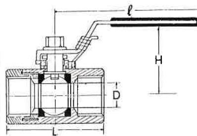
Fig. 2R224T, 2R233T 2000PSI Investment Cast 2PC Ball Valve Standard Bore
