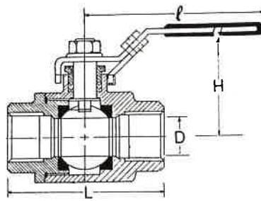
Fig. 2F124T, 2F133T 1000PSI Investment Cast 2PC Ball Valve Full Bore
