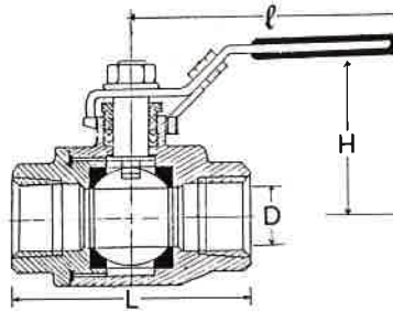
Fig. 2F224T, 2F233T 2000PSI Investment Cast 2PC Ball Valve Full Bore
